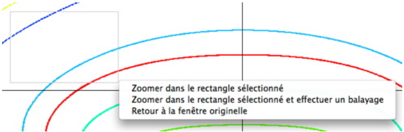
FIGURE 8 – Menu contextuel.
